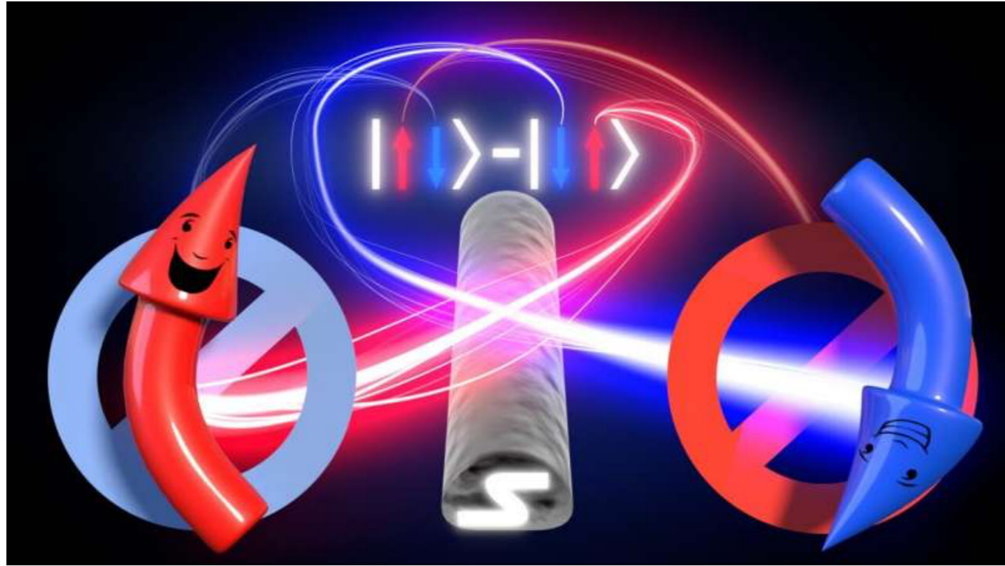
In contrast to parallel spin filters, for antiparallel spin filters electron pairs are all...
