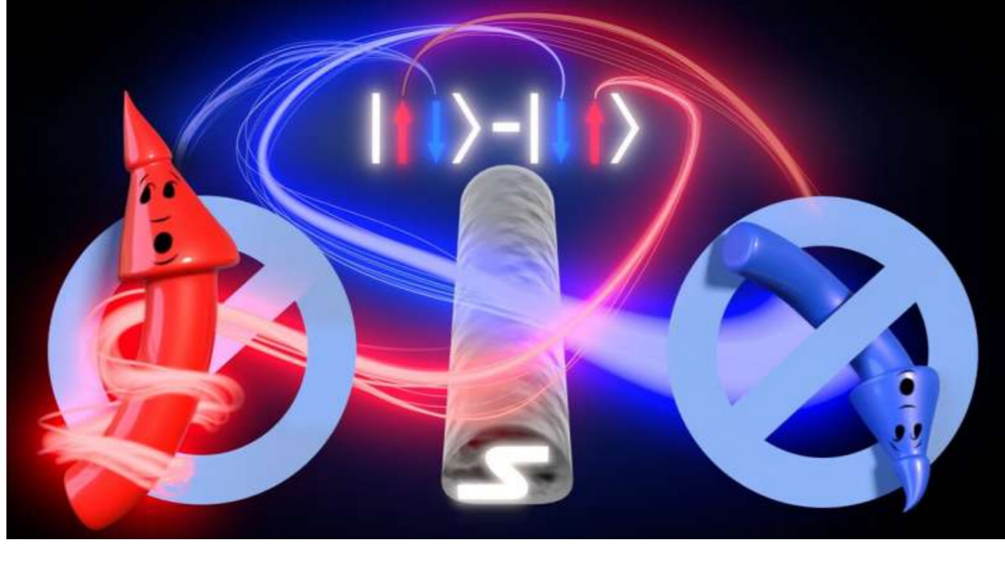
Electrons leave a (conventional) superconductor (S) only as pairs and only wit...
